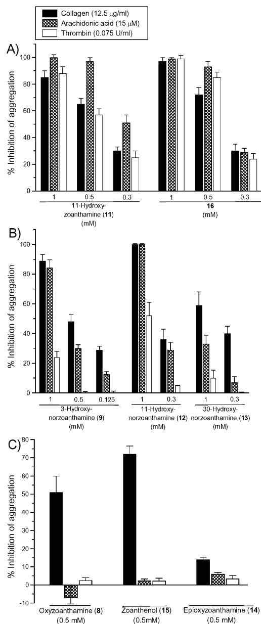
Figure 1. Effects of (A) 11-hydroxyzoanthamine (11) and 16, (B) 3-hydroxynorzoanthamine (9), 11-hydroxynorzoanthamine (12), and 30-hydroxynorzoanthamine (13); and (C) oxyzoanthamine (8), zoanthanol (15), and epoxyoanthamine (14) at different concentrations on washed human platelet aggregation induced by collagen, arachidonic acid and thrombin. Each value is the mean of 2–4 replicate assays. Vertical bars show standard errors of the mean.
